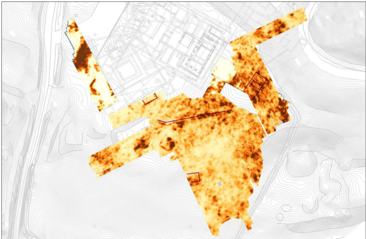
Fig. 3. La Pâture du Couvent. Graphic results of the GPR survey (top) and an interpretation (bottom), 2013-2014, constant time slice: 45 ns.
