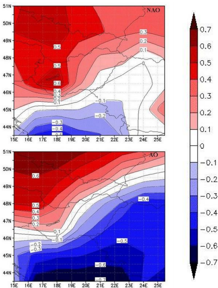
Figure 2. Correlation coefficient maps of daily NAO (upper panel) and AO (lower panel) indices with 2 meter air temperature anomalies (for which the 30 year mean of daily values are subtracted from the actual daily values) for January of 2013. Correlation coefficients exceeding 0.3 in absolute value are significant at 0.05 level.
