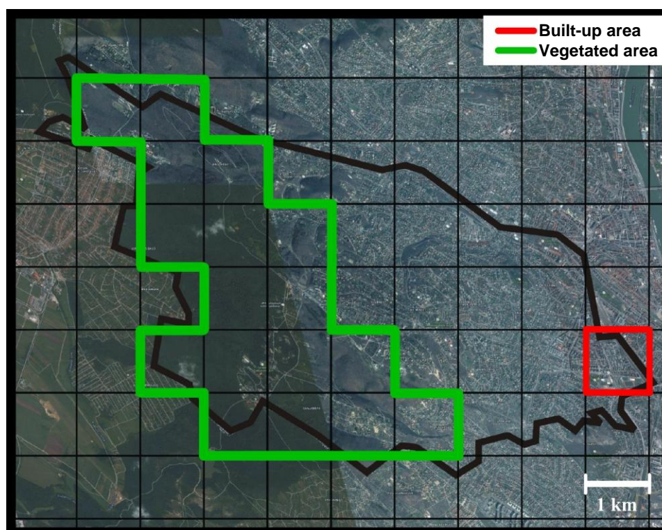
Fig. 1 Built-up and vegetated area of the 12th district of Budapest shown on the MODIS grid over the Google Earth satellite image.
