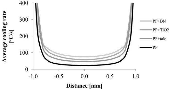
6. Figure The average cooling rate between the injection and ejection temperatures
