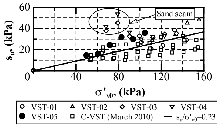
Figure 5. s_u vs. over-burdened stress ratio
