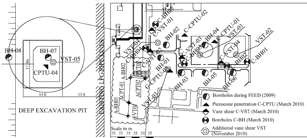
Figure 2. Layout plan of soil investigation for the project site
