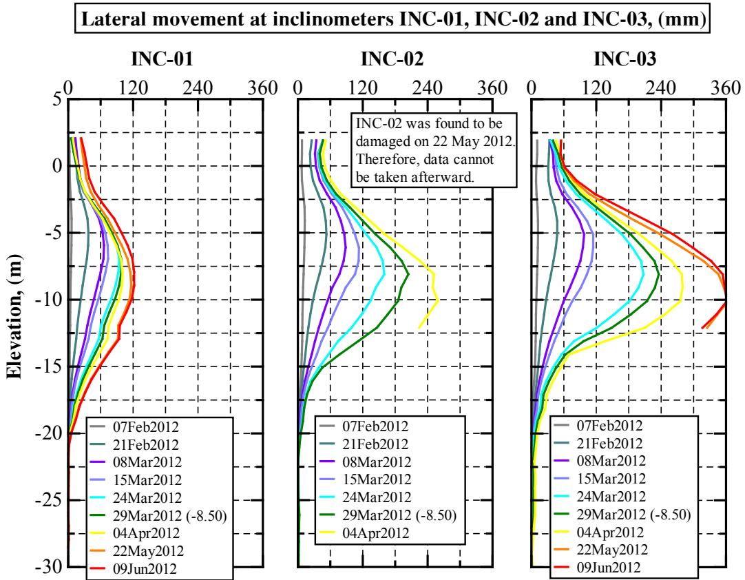
Figure 9. Monitoring data of lateral movement at all three inclinometers
