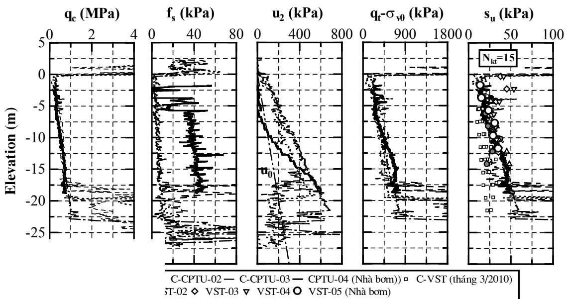
Figure 4. Piezocone penetration and field vane shear test results
