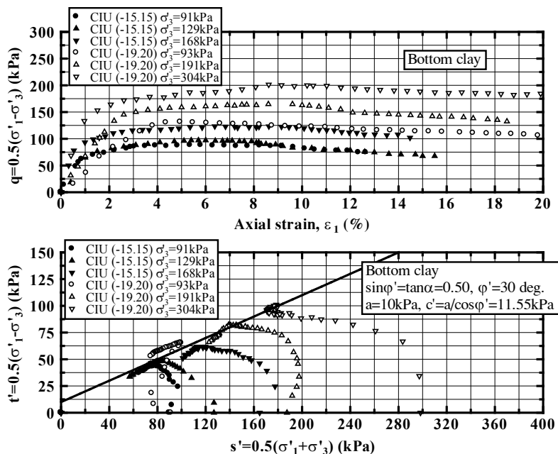
Figure 7. Triaxial test result for bottom soft clay
