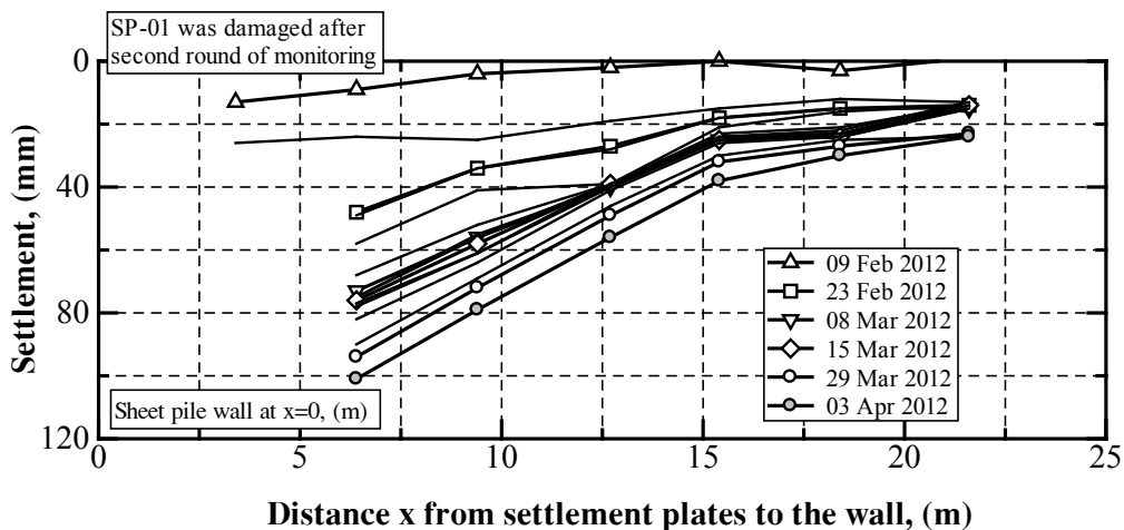
Figure 10. Monitoring data of surface settlement at plates SP-01 to SP-07
