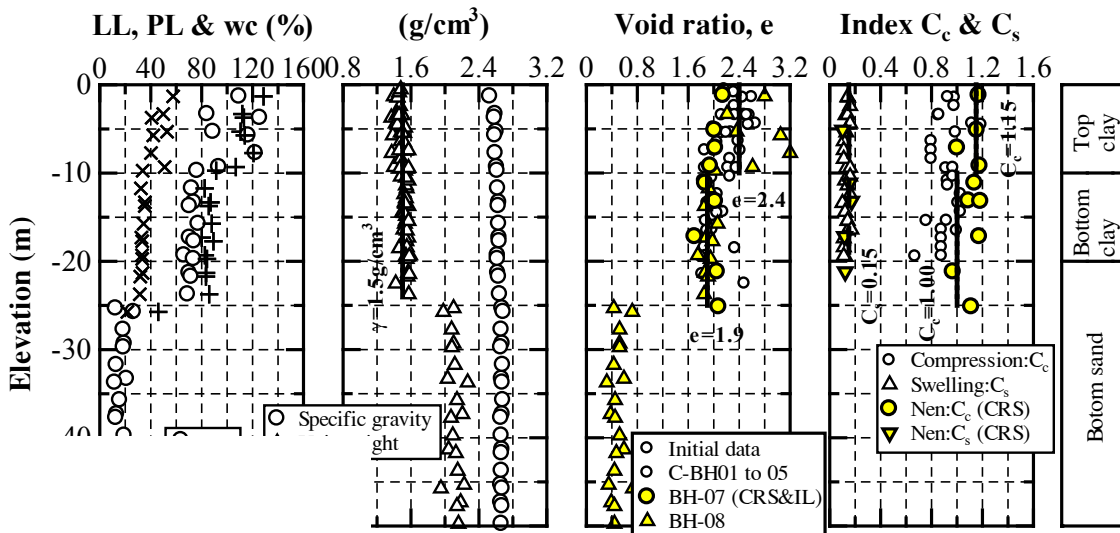
Figure 3. Physical mechanical properties
