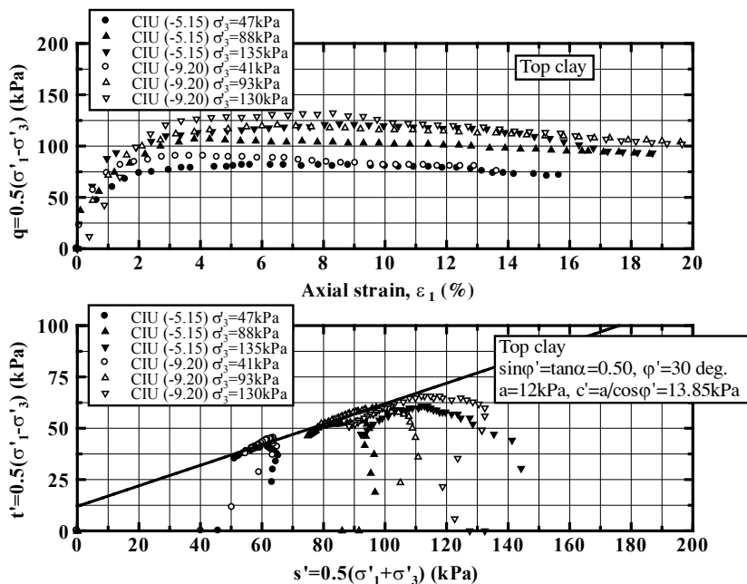
Figure 6. Triaxial test results for top soft clay
