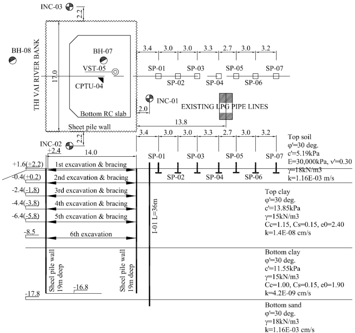
Figure 8. Arrangement of monitoring instrumentations (Dimension in m)
