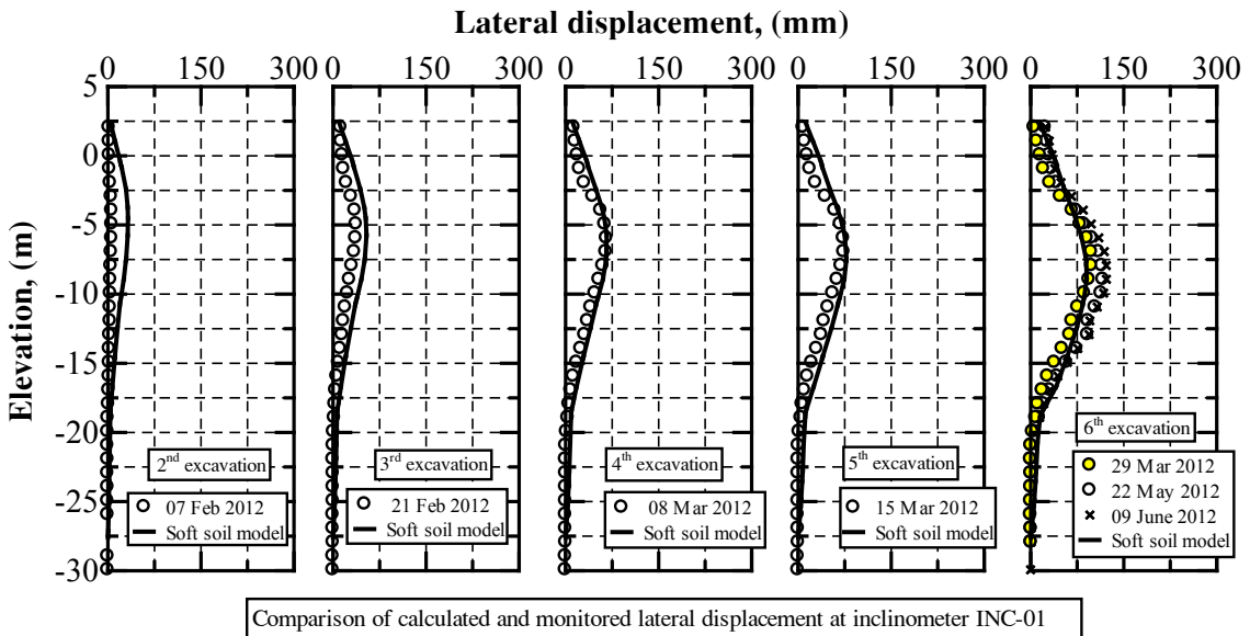
Figure 14. Comparison of calculated and monitored lateral movement at inclinometer
