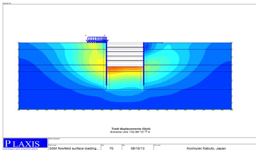
Figure 11. Shaded displacement at 6 th excavation
