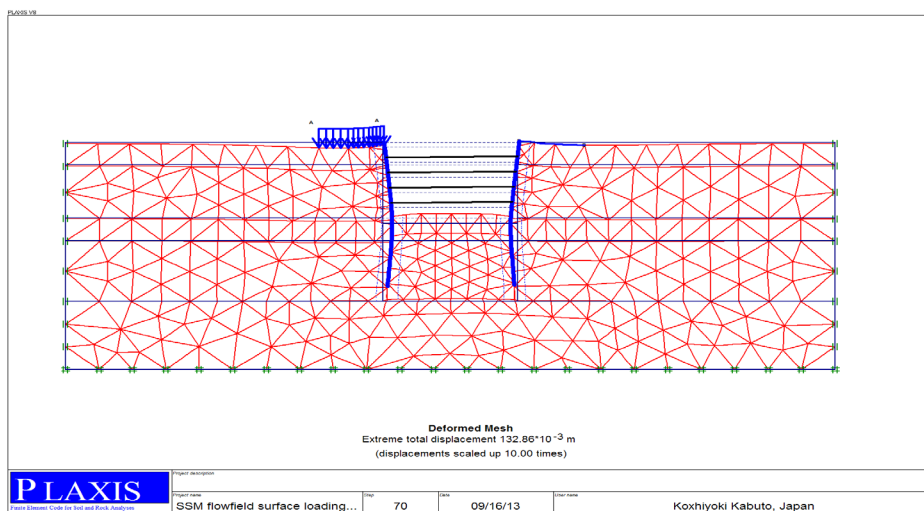
Figure 12. Deformed mesh at 6 th excavation
