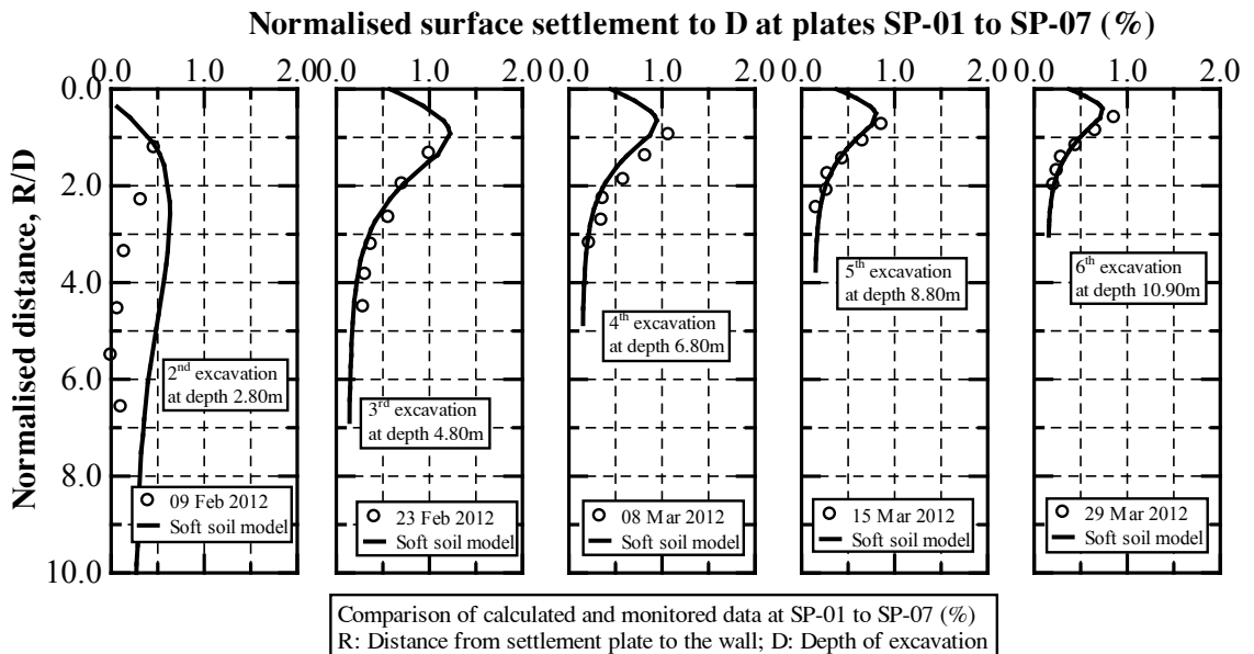
Figure 15. Comparison of calculated and monitored ground loss from the face of sheet pile wall
