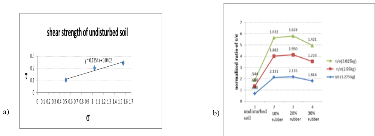
Figure 2. a) shear strength of undisturbed soil; b) normalized ratio \tau/\sigma
