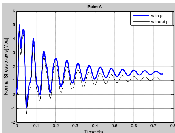
Figure 9. Normal stress \sigma_x at point A (with and without p)
