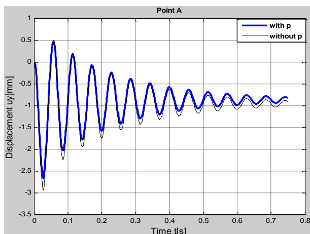
Figure 8. Displacement U_y at point A (with and without p)
