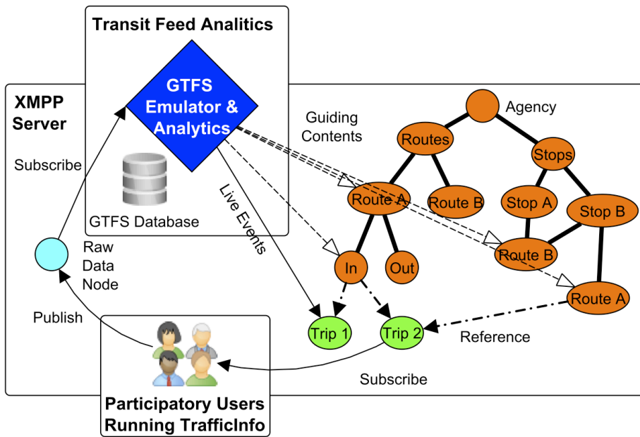
Figure 4: Smart timetable service architecture
