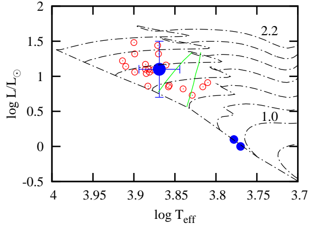
Figure 5. Possible locations of the three components in the KIC 4840675 system in the HR diagram (filled circles). The zero-age main sequence and several evolutionary sequences with solar composition (Bertelli et al. 2008) are shown. The sequences are spaced at intervals of 0.2M_{\odot} with masses of two tracks labeled. The solid lines mark the approximate location of the \gamma Dor variables.
