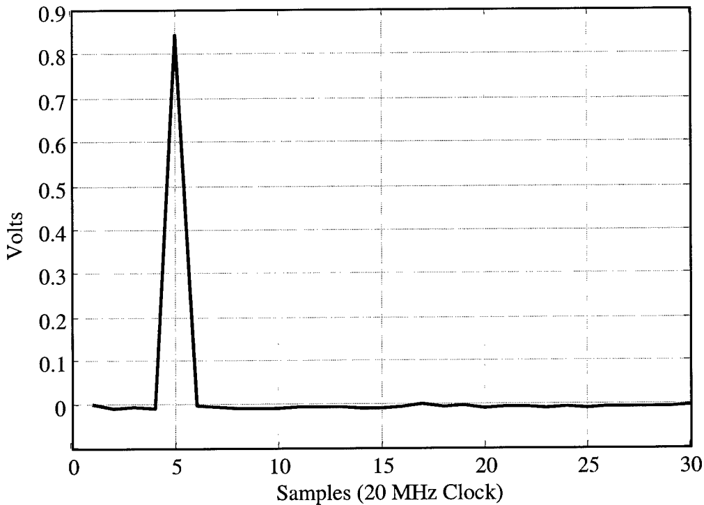
Figure 6. Digital Unit Minimum Delay Estimation.
