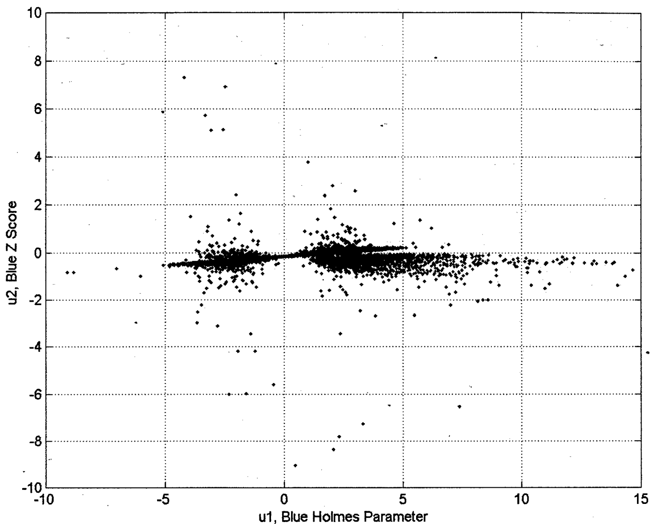
Figure 23. Projection of the input space into two dimensions by principal component analysis. The axes u_1 and u_2 correspond to the dimensions of the Holmes parameter and Z score for the blue bands respectively, as the eigenvectors of these two features corresponded to the two largest eigenvalues of the covariance matrix. The red data points represent components of the original missile features projected onto the new feature space and the black data points represent components of the background features projected onto the new space. There is a slight overlap between the two sets of data, but overall they appear to occupy different regions of the feature space. This result means that the features chosen have distinguishing characteristics that should provide a good discrimination capability to the RBF network.
