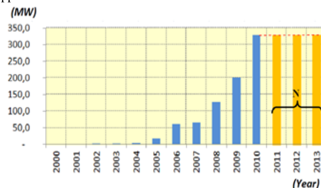
Illustration 6. Trend of Hungarian wind energy capacity [11, 12,13] (N - Not new installation)
