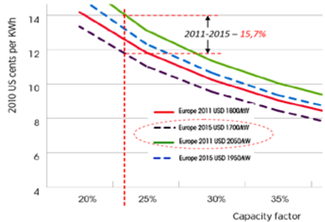
Illustration 12: The energy cost of wind power plants, and the utilization of the estimated price of investment (development for years 2011-2015) [10]
