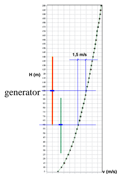
Illustration 4. Data from the measurement system on Figure 1. Wind speed difference 1,5 m/s, 60 and 100 m tower height
