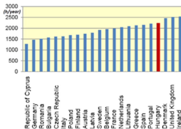
Illustration 8.Utilization of wind power plants (hn/year) of the EU's 24 countries [6]
