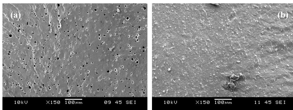
Figure 2. SEM pictures of the reference thermoplastic starch (a) and sample 2B (b).
