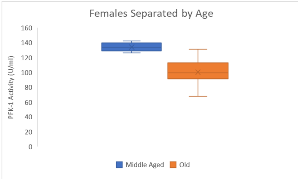
Figure 8: Females separated by age (n=22). P=0.00013. Quartiles are calculated with internal medians. Upper and lower whiskers represent the maximum and minimum distributions of the data. Unit (U) definition - One unit will convert 1.0 \mu mole of fructose-6-phosphate to fructose-1/6-bisphosphate minute at pH 8.2 at 39° C.
