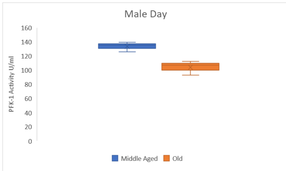
Figure 3: Male day middle aged moths (n=3) were compared to the male day old moths (n=3). P=0.0769. Quartiles are calculated with internal medians. Upper and lower whiskers represent the maximum and minimum distributions of the data. Unit (U) definition - One unit will convert 1.0 \mu mole of fructose-6-phosphate to fructose-1/6-bisphosphate per minute at pH 8.2 at 39° C.
