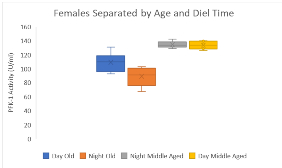
Figure 10: Females separated by age and diel time (n=23). Quartiles are calculated with internal medians. Upper and lower whiskers represent the maximum and minimum distributions of the data. Unit (U) definition - One unit will convert 1.0 \mu mole of fructose-6-phosphate to fructose-1/6-bisphosphate minute at pH 8.2 at 39° C.
