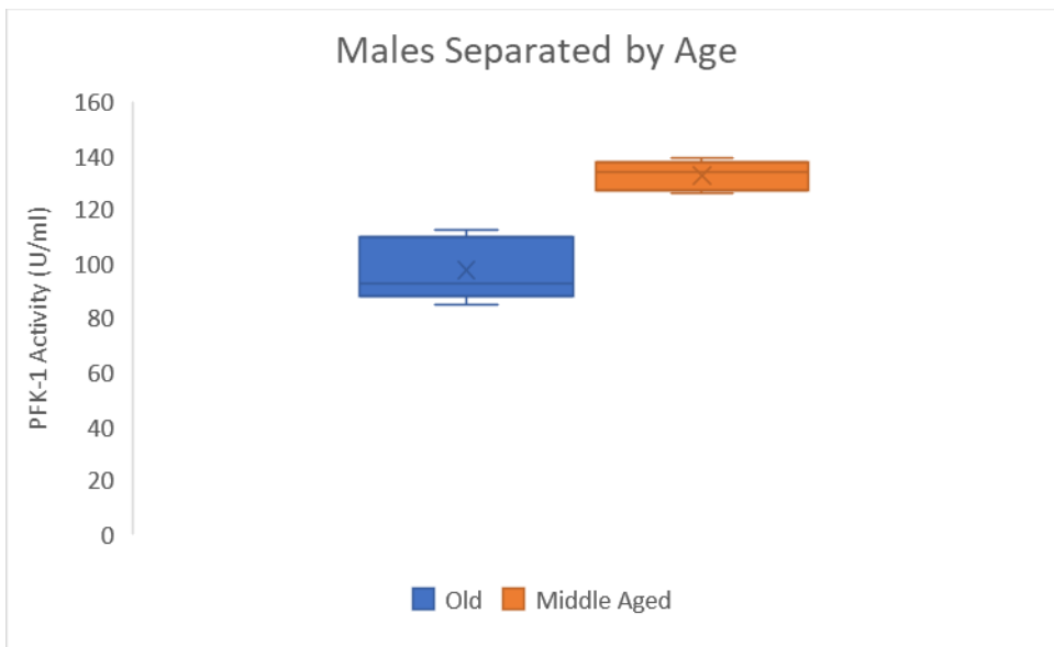
Figure 9: Males separated by age (n=10). P=0.0046. Quartiles are calculated with internal medians. Upper and lower whiskers represent the maximum and minimum distributions of the data. Unit (U) definition - One unit will convert 1.0 \mu mole of fructose-6-phosphate to fructose-1/6-bisphosphate minute at pH 8.2 at 39° C.
