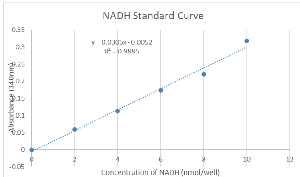
Figure 1: NADH standard curve with slope equation presented. Unit (U) definition - One unit will convert 1.0 \mu\text{mole} of fructose-6-phosphate to fructose-1/6-bisphosphate per minute at pH 8.2 at 39° C.
