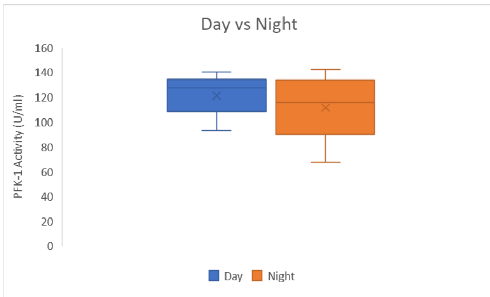
Figure 7: Day samples (n=12) were compared to the night samples (n=10). P=0.007. Quartiles are calculated with internal medians. Upper and lower whiskers represent the maximum and minimum distributions of the data. Unit (U) definition - One unit will convert 1.0 \mu mole of fructose-6-phosphate to fructose-1/6-bisphosphate minute at pH 8.2 at 39° C.
