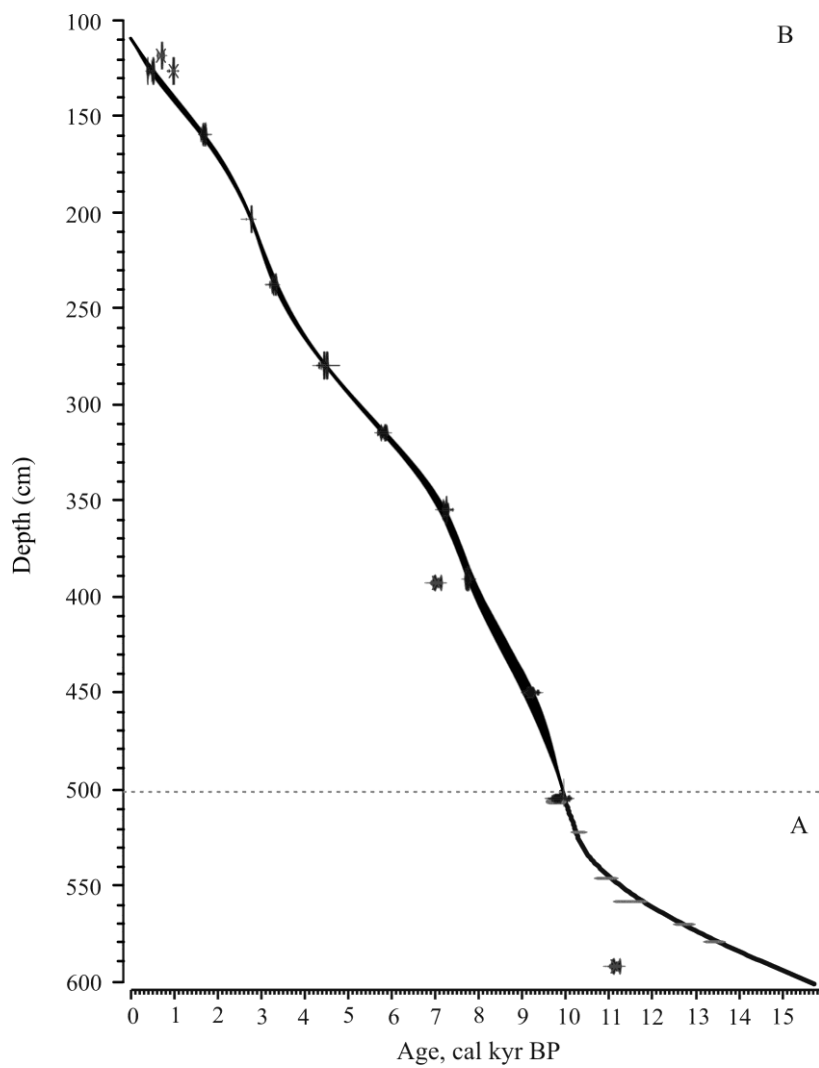
Figure 2. Age-depth models: (A) weighted non-linear polynomial regression for modelling the age-depth relationship in the late glacial and early Holocene part of the sediment record (600–502cm) and (B) a smoothing spline function in the Holocene part (505–111.14 cm) of the sediment record of Lake Brazi (Retezat Mts., South Carpathians).
