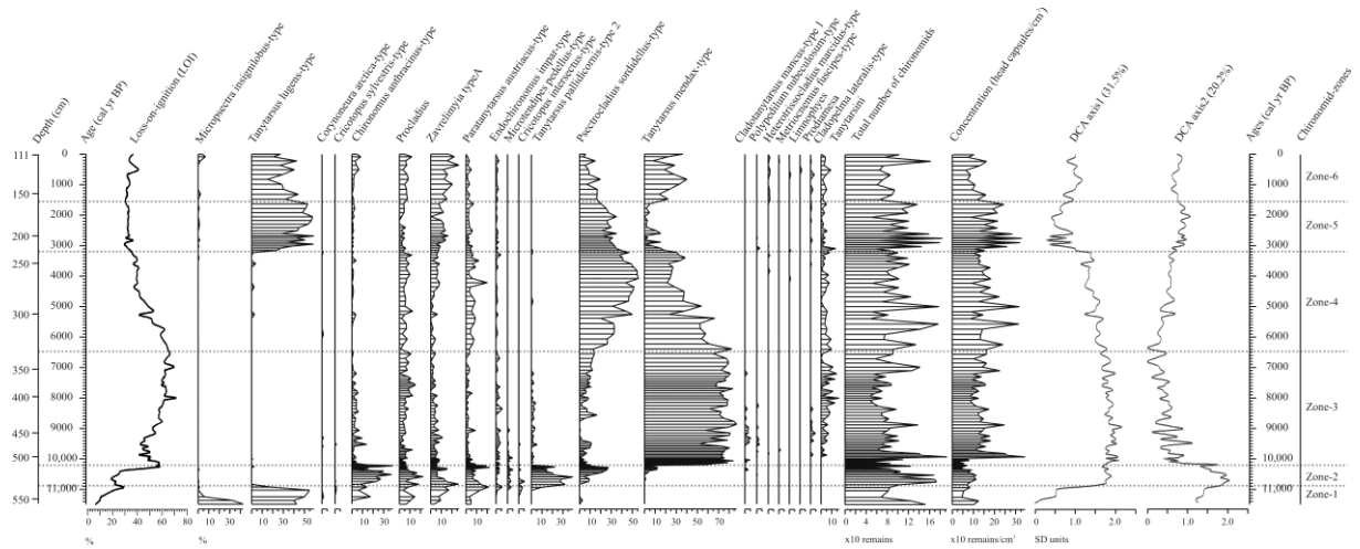
Figure 3. Chironomid relative abundance diagram including all chironomid taxa with Detrended Correspondence Analysis axes (DCA axis 1 and 2, with percentage variance explained by axes), loss-on-ignition (LOI) changes, and zones for the chironomid stratigraphy from Lake Brazi (Retezat Mts., South Carpathians).
