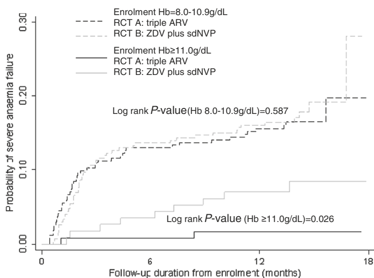
Figure 3 Kaplan-Meier failure curve showing anaemia failure (Hb < 8.0 g/dL) in RCT intervention arms, stratified by enrolment Hb level.
