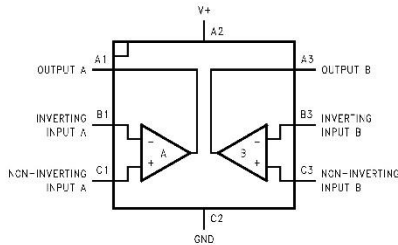
YPB Package 8-Pin DSBGA Top View
