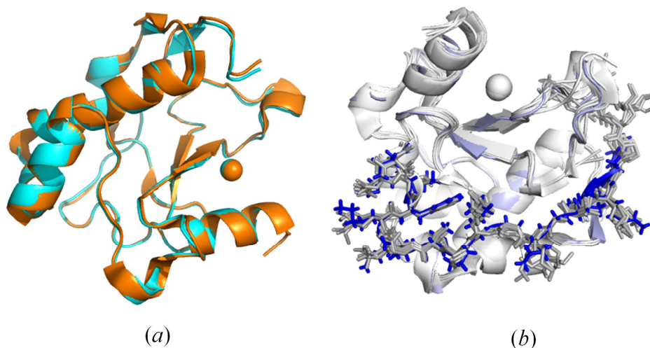
Fig. 7 a Structural alignment based on the identical amino acids of the \Delta N4-NCoIE7-C* (blue; PDB code: 3ZFK) and WT NCoIE7 (orange; PDB code: 1MZ8 6 ) shows good agreement between the structures of the two proteins. b Structural alignment of the N-terminal loops in selected NCoIE7 domains including the PDB structures 1M08 5 , 1MZ8 6 , 1PT3 3 , 1ZNS 7 , 1ZNV 7 , 7CEI 4 , 2IVH 8 , 2JAZ 9 , 2JB0 9 , 2JBG 9 and 3FBD 10 all in light grey and the \Delta 4-NCoIE7-C* in blue.
