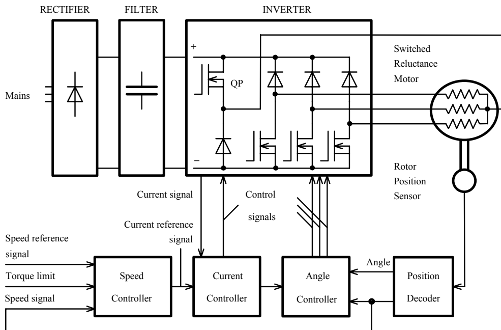
Fig.1. Block scheme of drive system
