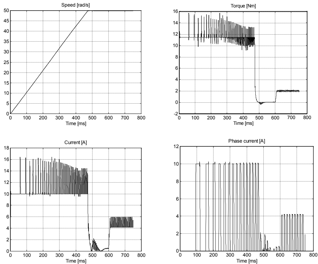
Fig. 3. Simulation results with model reference adaptive speed control.
