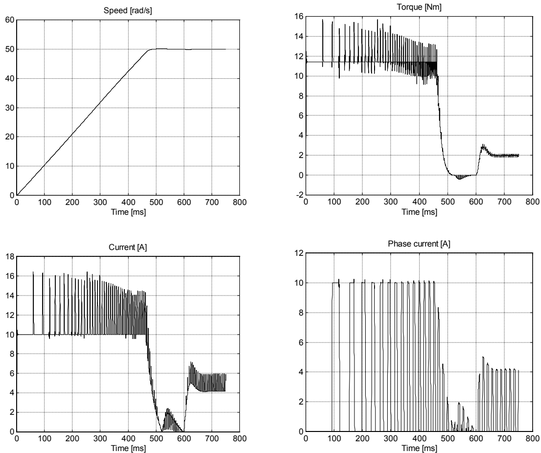
Fig. 2. Simulation results with speed controller of PDF-type.
