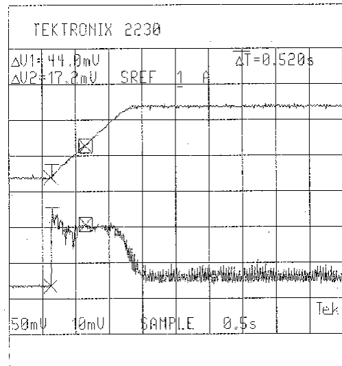
Fig. 5. Oscillograms of the speed and current, MRAC-type control.
