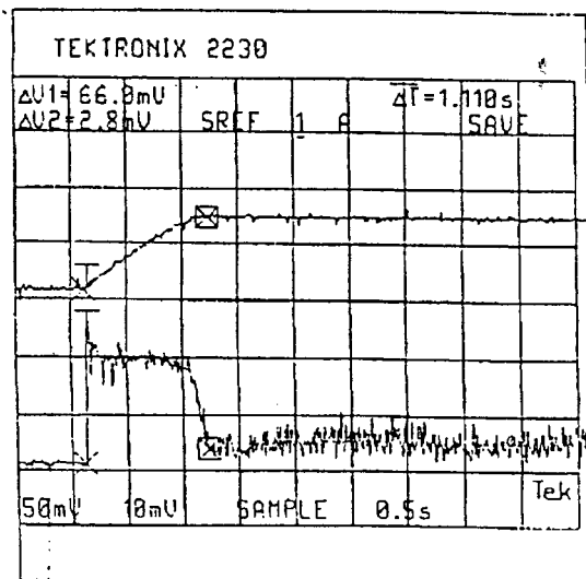
Fig. 4. Oscillograms of the speed and current, PDF-type control.
