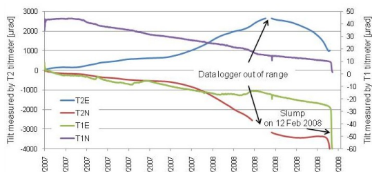
Figure 4 Tilt of the stable (T1) and unstable (T2) parts of the high bank before the landslide on 12 Feb 2008. T1N and T2N are the north, while T1E and T2E are the east components of the instruments. Tilt curves going to positive direction mean tilts toward to east and north
