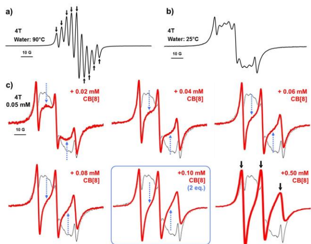
Figure 1. EPR spectra in water solution of a) 4T at 363 K, b) 4T at 298 K, c) 4T in the presence of increasing amounts of CB[8] highlighting the absence of noticeable changes above 2 equivalents of CB[8].
