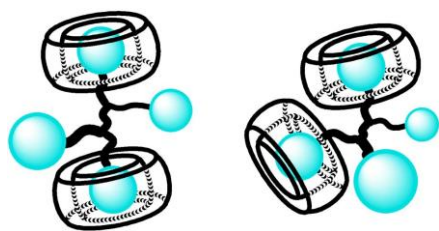
Scheme 2. Two possible modes of inclusion for the complex 4T@CB[8]_2 .
