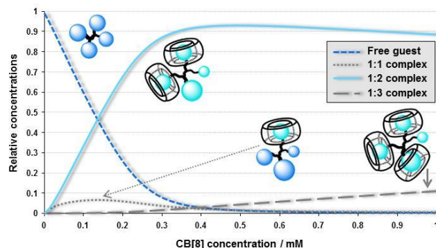
Figure 2. Products distribution for the binding of tetranitroxide 4T (0.05 mM) with CB[8] in water.
