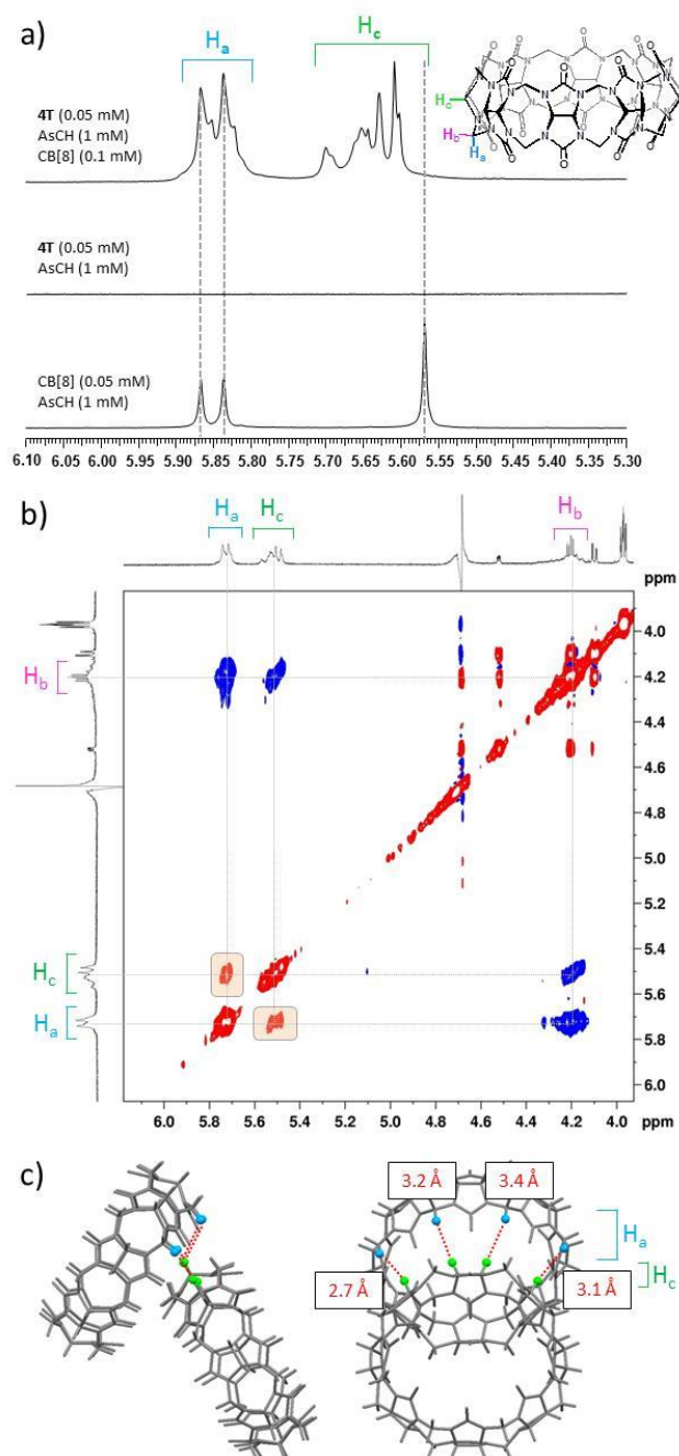
Figure 3. (a) Excerpts of the 600 MHz 1 H NMR spectra of the reduced form of 4T (hydroxylamines) in the absence and in the presence of CB[8] in water showing the splitting of the singlet of the methine protons of CB[8]. (b) Part of the 2D-ROESY spectrum of a mixture of 4T (0.05 mM) and CB[8] (0.1 mM) with ascorbic acid (1 mM, 300K, mixing time: 800 ms). (c) Part of the CB[8] supramolecular triangle (X ray structure of ref. 21) featuring two CB[8] interacting by multiple C-H...O interactions as a mean to measure H...H contacts between H_a(CB[8])_{TOP} and H_c(CB[8])_{BOTTOM} .
