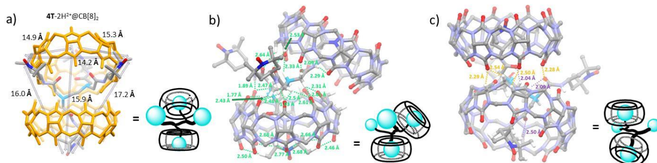
Figure 4. (a) Calculated structure (B 3 LYP/6-31G (d)) of the most stable conformer of the 1:2 complex of tetranitroxide 4T in its doubly charged state with CB[8]. The large interspin distances (> 14 Å) correlate well with experimental data (EPR). Host-guest (b) and host-host (c) hydrogen bonds and weak interactions found in the 1:2 complex of 4T with CB[8] (see text and supporting information for details).
