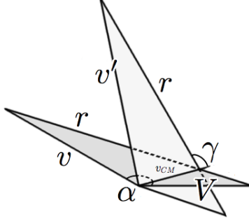
Figure 2: \vec{v}, \vec{V} : incoming velocities; \vec{v}_{CM} : velocity of center of mass; \vec{r} = \vec{v} - \vec{v}_{CM} : velocity of the first particle relative to the center of mass; \vec{v}' : velocity of the first particle after rebound; \alpha = \angle(\vec{v}, \vec{V}) : angle between incoming velocities; \gamma = \angle(\vec{r}', \vec{v}_{CM}) : angle of rebound.
