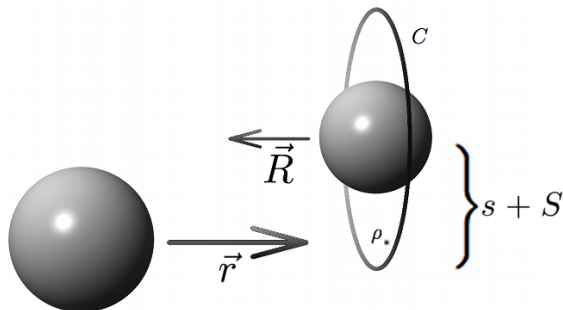
Figure 1: \vec{r}, \vec{R} : velocities relative to the center of mass. C : circle of radii s + S centered on the second particle in the plane perpendicular to \vec{r} . \rho : point where the line of motion of the first particle intersects circle C .
