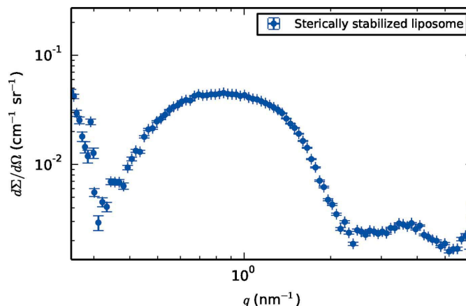
Figure 4 Small-angle X-ray scattering curve of a sterically stabilized liposome.
