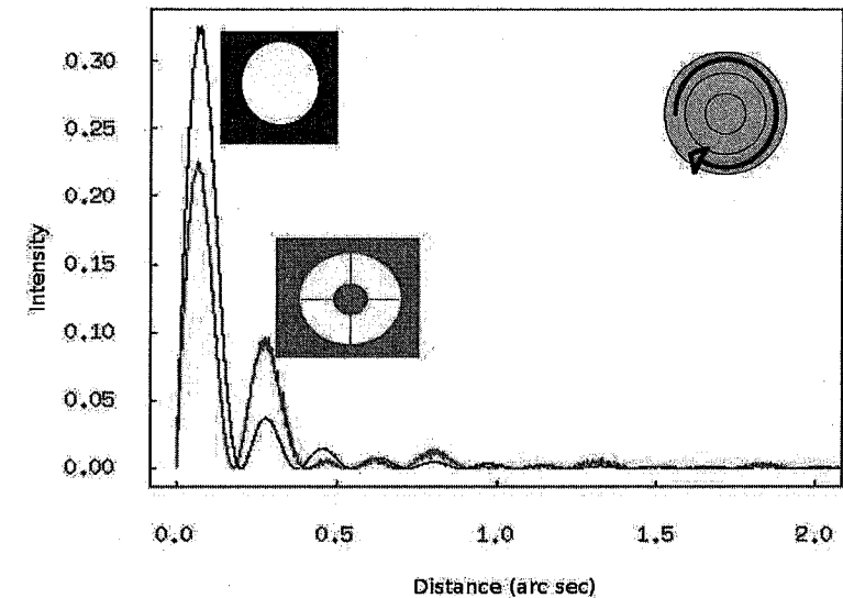
Figure 2. Amount of the total light scattered to a given distance from the center of the Airy disk. The unocculted system has a higher peak and lower sidelobes; note that much light is scattered from the Airy disk to the first sidelobes by the secondary mirror.
