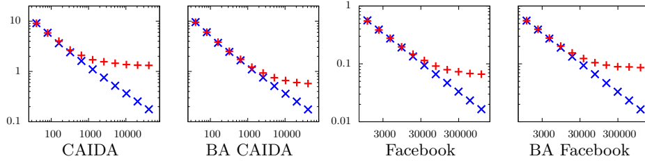
Fig. 7. Relative safety loading (for 0.999) as a function of size for random samples (red +) and for binomial distributions having the same average risk (blue x).
