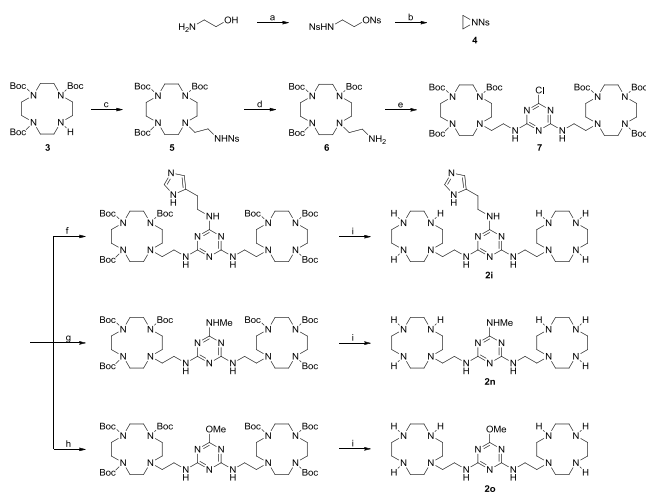
Scheme 1 Preparation of the cleaving agents 2i , 2n and 2o . Reagents and conditions: (a) 4-nitrobenzenesulfonyl chloride, pyridine, \text{CH}_2\text{Cl}_2 , (b) KOH, \text{H}_2\text{O} , \text{CH}_2\text{Cl}_2 , (c) 4 , MeCN, (d) thioglycolic acid, DBU, DMF, (e) cyanuric chloride, DIPEA, MeCN, (f) histamine, DIPEA, MeCN, (g) methylamine, EtOH, (h) NaOMe, MeOH, (i) TFA, \text{CH}_2\text{Cl}_2 , MeOH.
