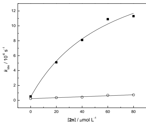
Fig. 5. Pseudo first-order rate constants for the cleavage of UpU (■) and ApA (○) as a function of the concentration of the cleaving agent 2n at 90\text{ }^\circ\text{C} , \text{pH}^* = 6.57 , I(\text{NaClO}_4) = 0.10\text{ mol L}^{-1} , [\text{UpU}] = [\text{ApA}] = 5.0\text{ } \mu\text{mol L}^{-1} .
