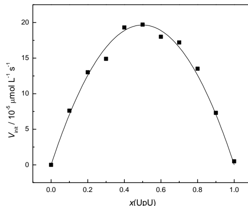
Fig. 6 Initial rate for the cleavage of UpU by 2n at 90\text{ }^\circ\text{C} , \text{pH}^* = 6.39 , I(\text{NaClO}_4) = 0.10\text{ mol L}^{-1} , [\text{UpU}] + [\mathbf{2n}] = 50\text{ } \mu\text{mol L}^{-1} .
