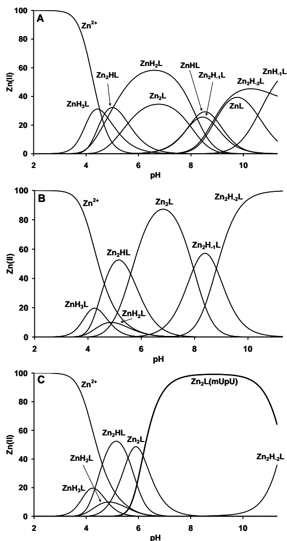
Fig. 2 Species distribution curves for the Zn^{II} complexes in the Zn^{II} / L / mUpU = 1/1/0 (A), 2/1/0 (B) and 2/1/1 (C) systems ( T = 25\text{ }^\circ\text{C} , I (NaCl) = 0.1\text{ mol L}^{-1} , [L] = 1\text{ mmol L}^{-1} ).
