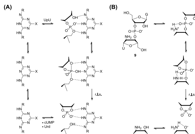
Scheme 5 Proposed mechanisms for (A) cleavage of UpU by 2h , 2i , 2n and 2o and (B) spontaneous cleavage of guanylyl-(3',3')-(2'-amino-2'-deoxyuridine) ( 9 ).
