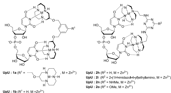
50 Fig. 1 Complexes of UpU with bi- and trinuclear Zn II chelates of 1,5,9-triazacyclododecane ( 1a and 1b ) and cyclen ( 2h , 2i , 2n and 2o ).
