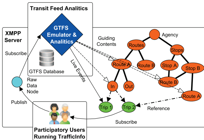
Fig. 2. Demonstration System Architecture
