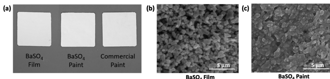
Figure 1. Radiative cooling coatings and SEM images. (a) BaSO 4 film sample, BaSO 4 -acrylic paint sample, and white commercial paint. The BaSO 4 film is 150 μm thick on a silicon wafer. The BaSO 4 paint and commercial paint are freestanding samples with a thickness of 400 μm. All samples are 5 cm squares. (b) BaSO 4 film sample under SEM. (c) BaSO 4 -acrylic composite paint sample with a 60% filler concentration under SEM. (b, c) Particle size distribution (398 ± 130 nm) was estimated based on the SEM images. Air voids were introduced in both the BaSO 4 film and the BaSO 4 paint.
