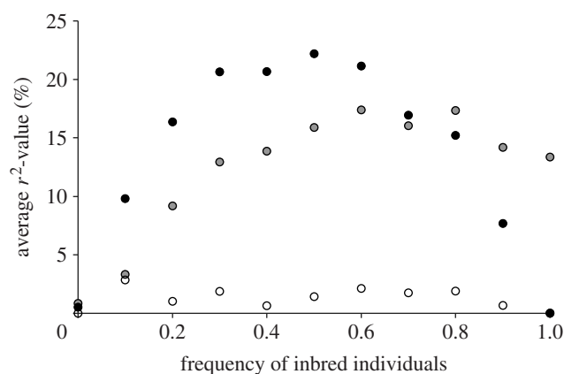
Figure 2. Relationship between the strength of the heterozygosity–heterozygosity correlation across markers and the proportion of inbred individuals. The proportion of inbred individuals varies between 0 and 100% in 10% intervals and data are presented for simulations where all inbred individuals are the progeny of second cousins ( F=0.016 , open circles) first cousins ( F=0.063 , black circles) and an equal mixture of the two (grey circles).
