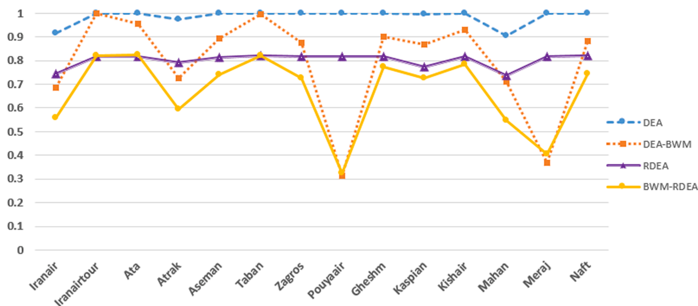
Fig. 2. Efficiency scores generated by DEA, BWM-DEA, RDEA and BWM-RDEA models.
