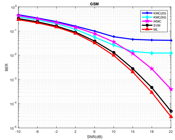
FIGURE 7. BER performance analysis of KMC detector, IKMC detector, proposed SVM aided detector and ML detector of GSM-VLC system with system configuration: N_t = 8 , N_r = 4 , n_t = 2 , M = 2 .
