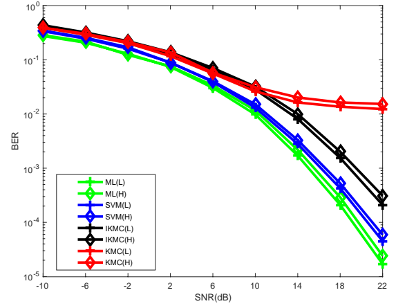
FIGURE 13. BER performance analysis of KMC detector, IKMC detector, proposed SVM aided detector and ML detector of GSM-VLC system with different vertical distances between LEDs and PDs: 2 m and 1 m.
