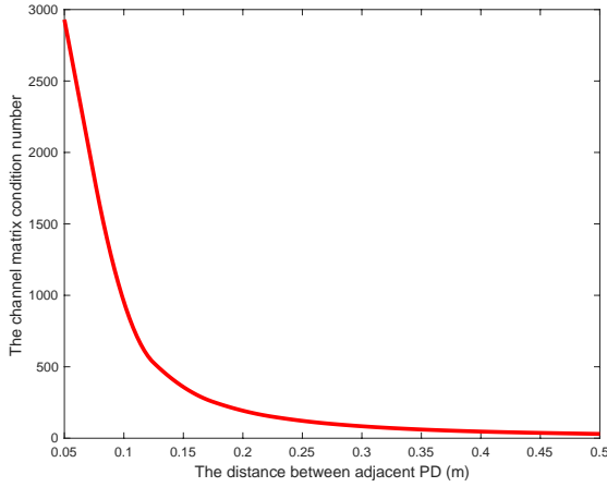
FIGURE 9. The relationship between channel matrix condition number and the PDs spacing.
