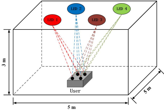
FIGURE 1. Conceptual diagram of indoor VLC system: N_t = N_r = 4 , \bar{L} = \bar{W} = 5 m, \bar{H} = 3 m.
