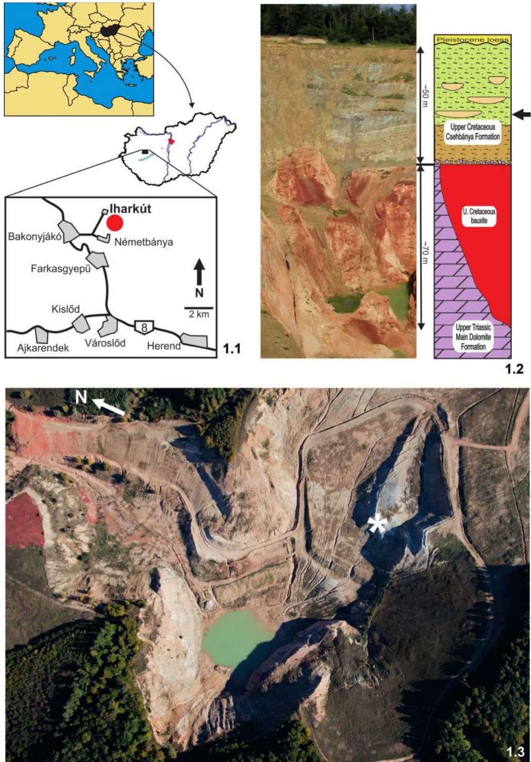
FIGURE 1. (1) Location map of the Iharkút vertebrate locality (Upper Cretaceous [Santonian] Csehbánya Formation, Bakony Mts, western Hungary). (2) Schematic section of the open-pit Iharkút (after Ósi and Mindszenty, 2009). The black arrow indicates the position of the bone-yielding beds that, among other fossils, provided the fragmentary skull referred to Hungarosaurus sp. (in this work) and the associated Hungarosaurus skeletons. (3) The Iharkút locality from a bird's eye view. Asterisk marks the site where the fragmentary skull was found.
