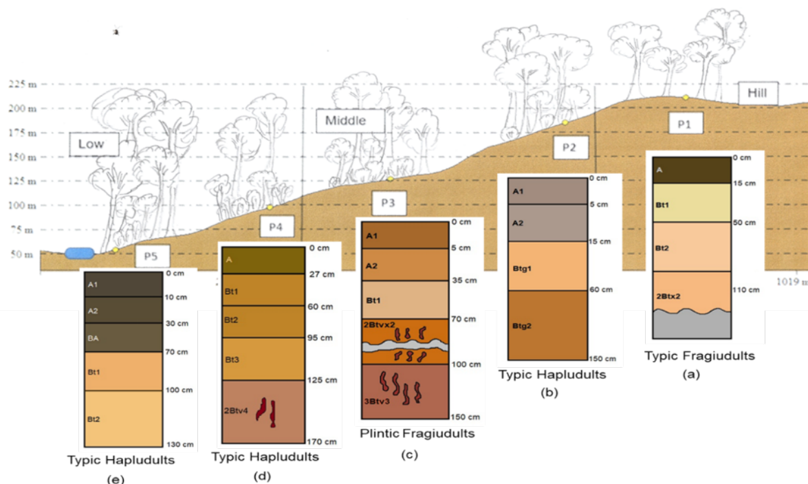
Fig. 3. Crosssection of pedon location along toposequence: (a) top (b) upper middle slope (c) lower middle slope (d) lower slope (e) foot slope.
