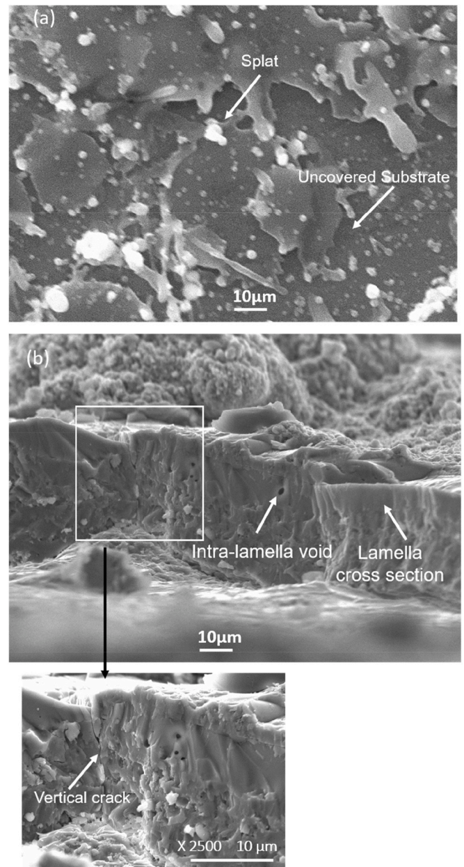
Fig. 5. SE scanning electron micrograph of (a) molten S-YAG topcoat splats collected on mirror polished AISI 304 stainless steel showing the splat morphology and spread after impact (b) fractograph of S-YAG topcoat showing lamella cross-section and intra-lamella void, with a higher magnification image in the inset.
