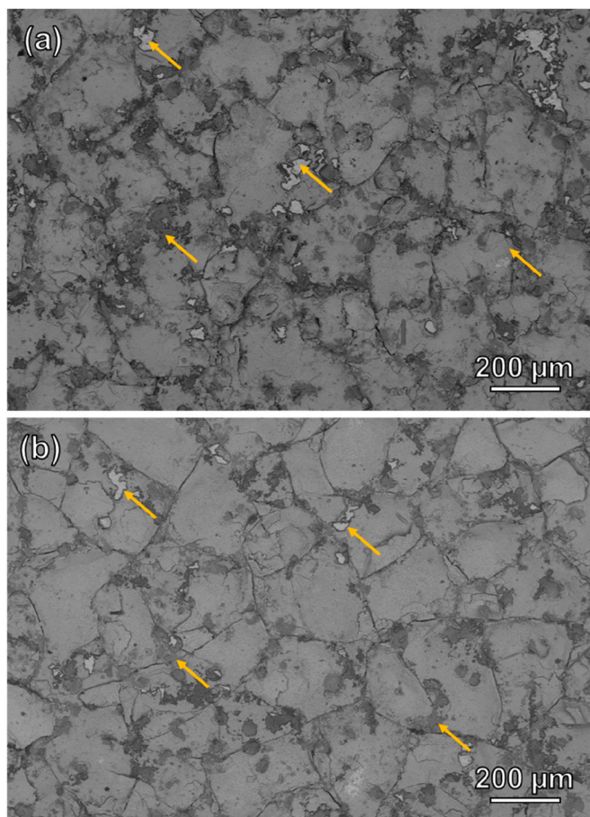
Fig. 10. BSE scanning electron micrograph showing spallation sites (arrows) on the surface of the (a) thermally cycled SP-YAG topcoat (b) thermally cycled S-YAG topcoat, respectively.
