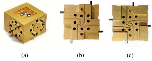
Fig. 5. The fabricated filtering coupler. (a) the overall view. (b) the upper part. (c) the lower part.
