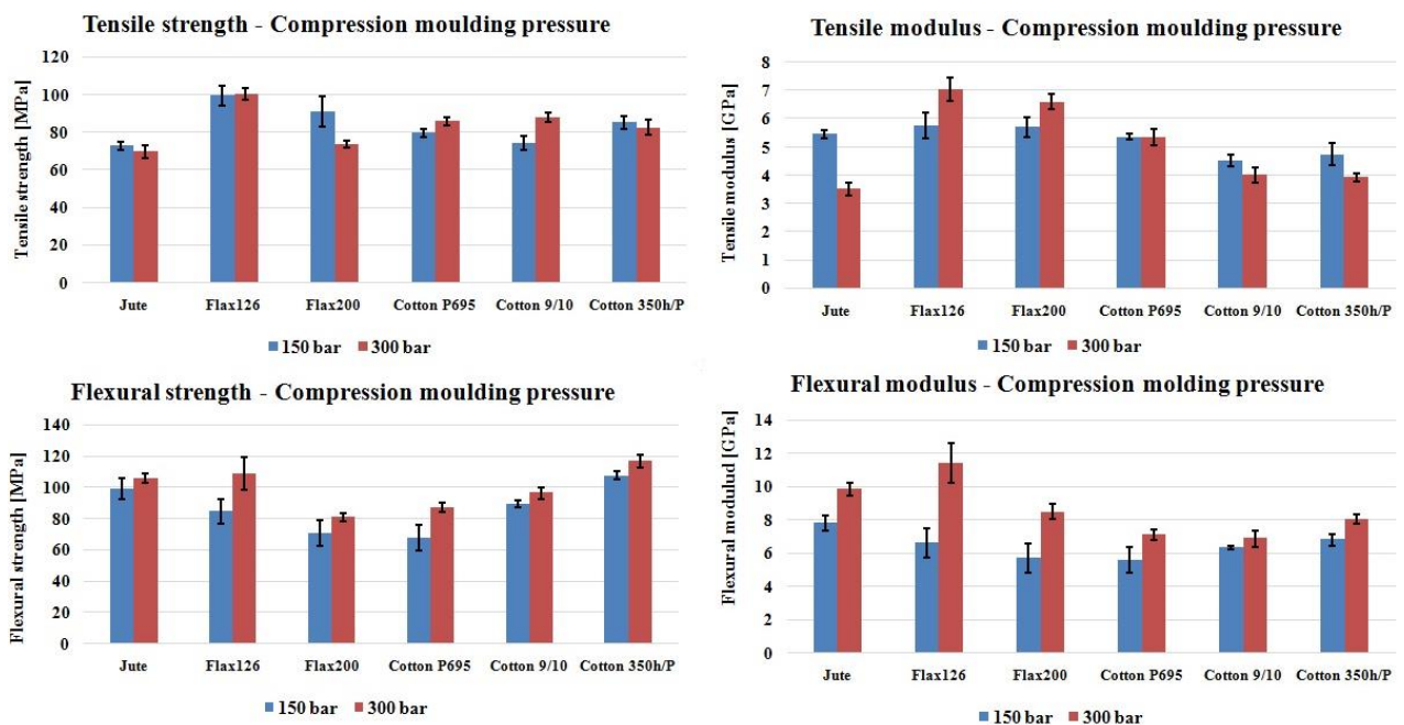
Figure 3. Mechanical properties of the composites
