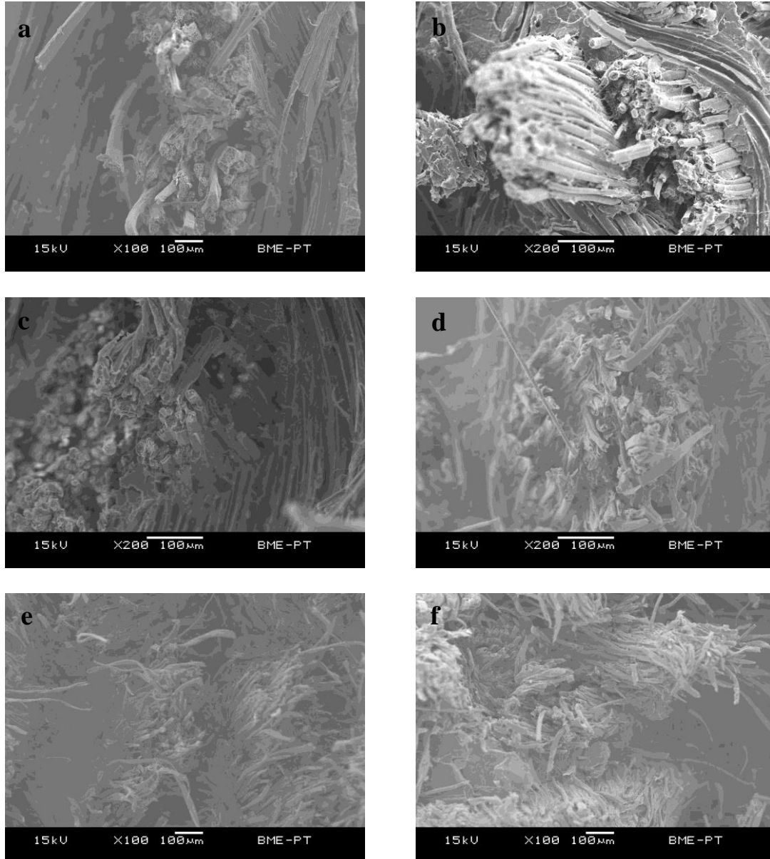
Figure 4. SEM images of the composite made with 150 bar a) PLA/Jute, b) PLA/Flax126, c) PLA/Flax200, d) PLA/Cotton P695, e) PLA/Cotton 9/10, f) PLA/Cotton 350h/P
