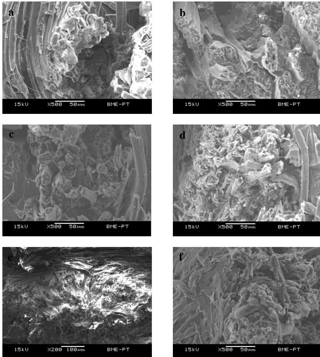
Figure 5. SEM images of the composite made with 300 bar a) PLA/Jute, b) PLA/Flax126, c) PLA/Flax200, d) PLA/Cotton P695, e) PLA/Cotton 9/10, f) PLA/Cotton 350h/P
