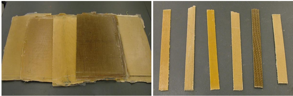
Figure 2. PLA/natural fibre composites made with compression moulding (left) and the test specimens (right)
