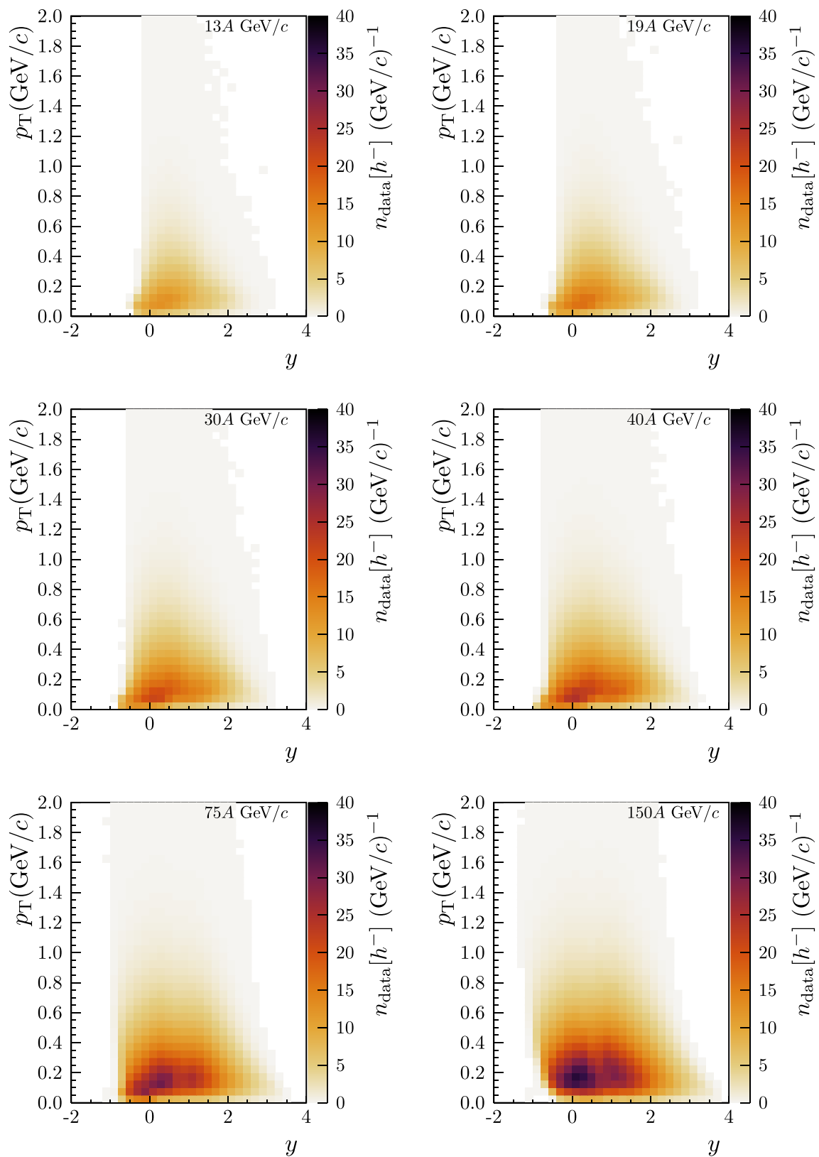
Fig. 7 Uncorrected double-differential spectra n[h^-]^{raw}/\Delta y/\Delta p_T of negatively charged hadrons produced in the 5% Ar+Sc collisions with the smallest E_{PSD} energy at beam momenta of 13A, 19A, 30A, 40A, 75A and 150A GeV/c
