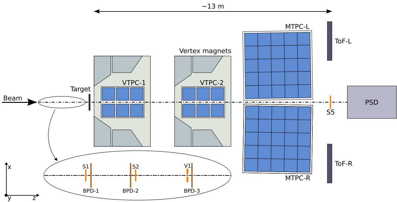
Fig. 1 The schematic layout of the NA61/SHINE experiment at the CERN SPS [1] showing the components used for the Ar+Sc energy scan (horizontal cut, not to scale). The trigger detector configuration upstream of the target is shown in the inset. Alignment of the chosen coordinate system is shown on the plot; its origin lies in the middle of
