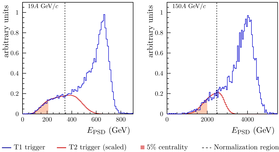
Fig. 3 Event centrality selection using the energy E_{PSD} measured by the PSD calorimeter. Distributions are shown of measured E_{PSD} for minimum-bias selected (blue histograms) and T2 selected (red histograms) events for 19A (left plot) and 150A GeV/c (right plot) beam momenta. Histograms are normalized to agree in the overlap region
