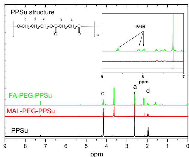
Fig. 1 1 H-NMR spectra of PPSu, MAL–PEG–PPSu and FA–PEG–PPSu
