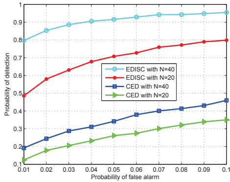
Fig. 4: ROC curves for classical ED and ED with imperfect cancellation when \text{ISNR} = -10 dB, E_s = 0 dB and \sigma_w^2 = -7 dB.
