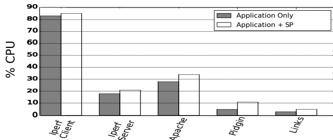
Fig. 3: CPU overhead of the SP
