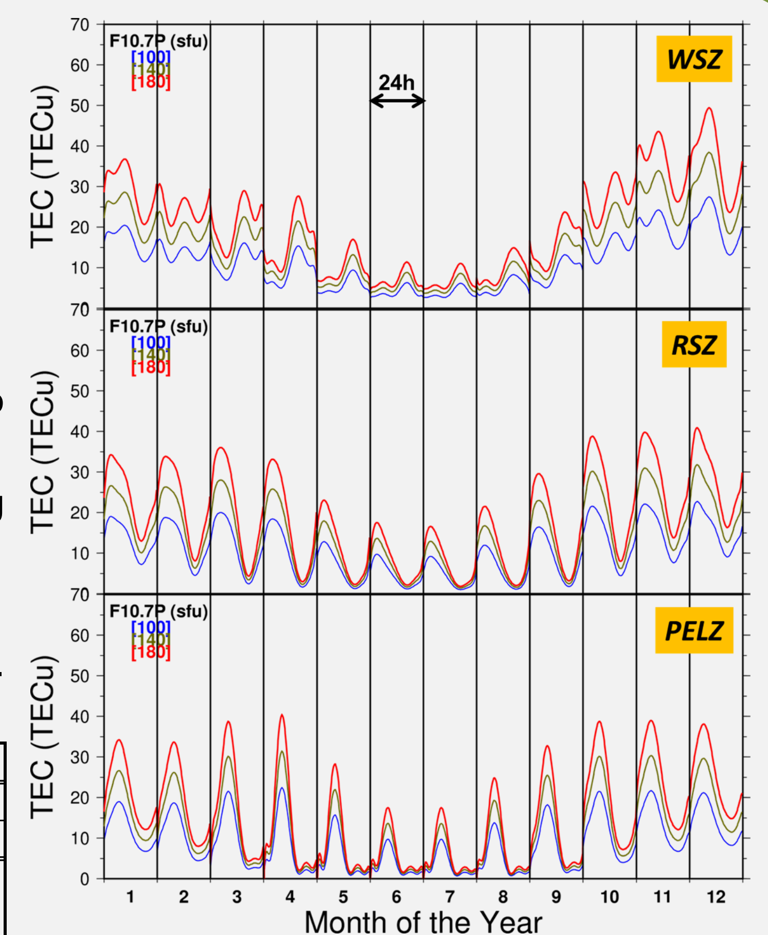
Figure 3: Monthly climatological of the TEC over Antarctica over PELZ, RSZ and WSZ (see figure 2) for different level of solar activity: high (red), transition (green) and low (blue) solar activity level.
