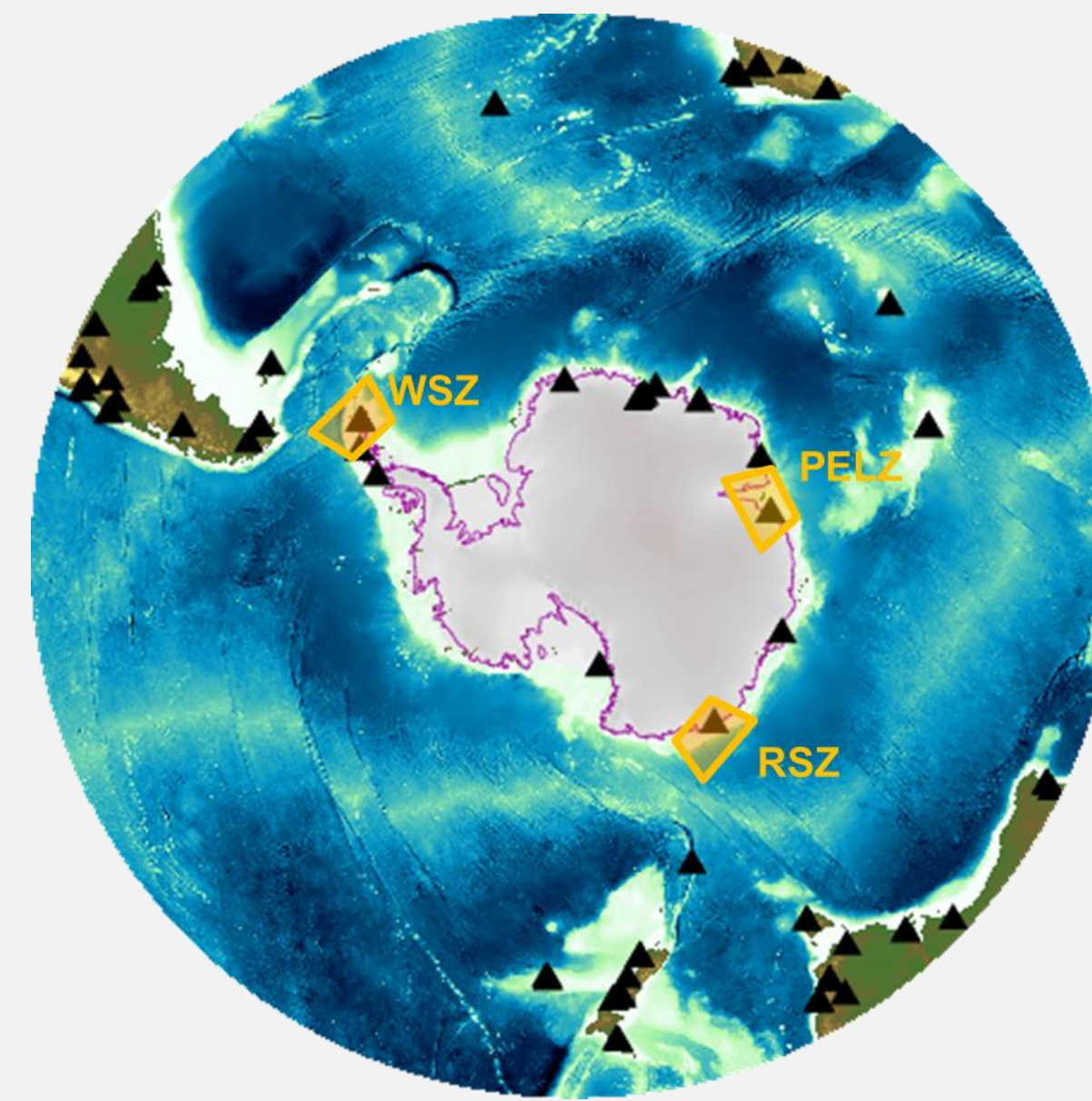
Figure 2: GNSS network in this study. The black triangles are the GNSS stations processed for the period of interest. In orange are represented the 3 zones presenting the different climatological patterns described in section 3.
