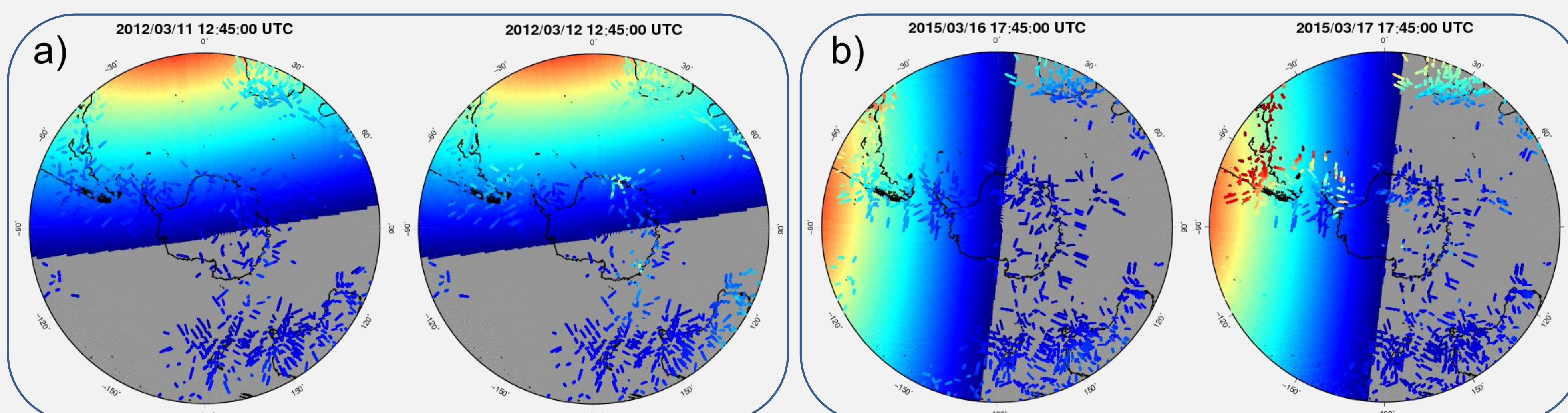
Figure 4: Impact of two CMEs on ionospheric Total Electron Content over Antarctica. The grids are the solar zenith angle for the days and hours of interest. The dots are the TEC values at IPPs estimated from the GNSS network described in section 2. a) Event on March 12, 2012. Geomagnetic indices K_p = 6 ; A_p = 94 b) Event on March 17, 2015. Geomagnetic indices K_p = 8 ; A_p = 179 Also shows the quiet ionospheric conditions during the day before the storm.
