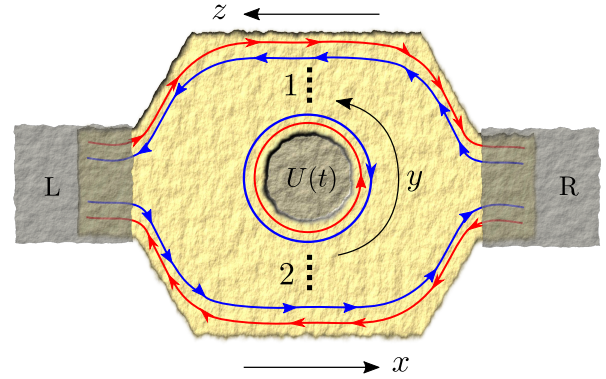
FIG. 1. Antidot (central grey area) realized in a narrow QSH bar (yellow) coupled to both the two edges in a two-terminal configurations (left (L) and right (R) grey rectangles). Tunnel junction 2 is created at x = 0, y = 0 with tunnel junction 1 at y = \pi R, z = 0 . Spin up and spin down edge states are depicted in red and blue respectively. The antidot is driven by a time-dependent potential U(t) .
