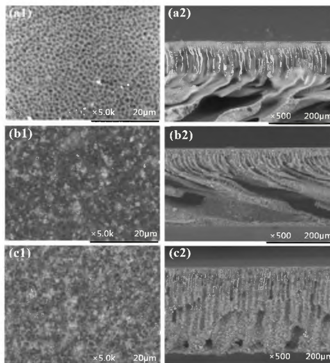
Fig. 5. SEM images of top surface (magnification of 5000 ×) and cross section (magnification of 500×) of PES membranes prepared from different nanoparticles loadings, (a) PES, (b) PES/HMO-1 and (c) PES/HMO-2 membrane
