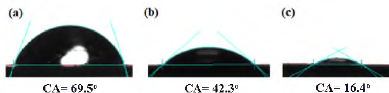
Fig. 4. Water contact angle of membranes, (a) PES, (b) PES/HMO-1 and (c) PES/HMO-2 membrane
