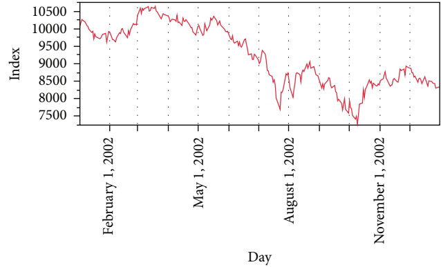
FIGURE 2: Unprocessed data for year 2002 of DJI.
