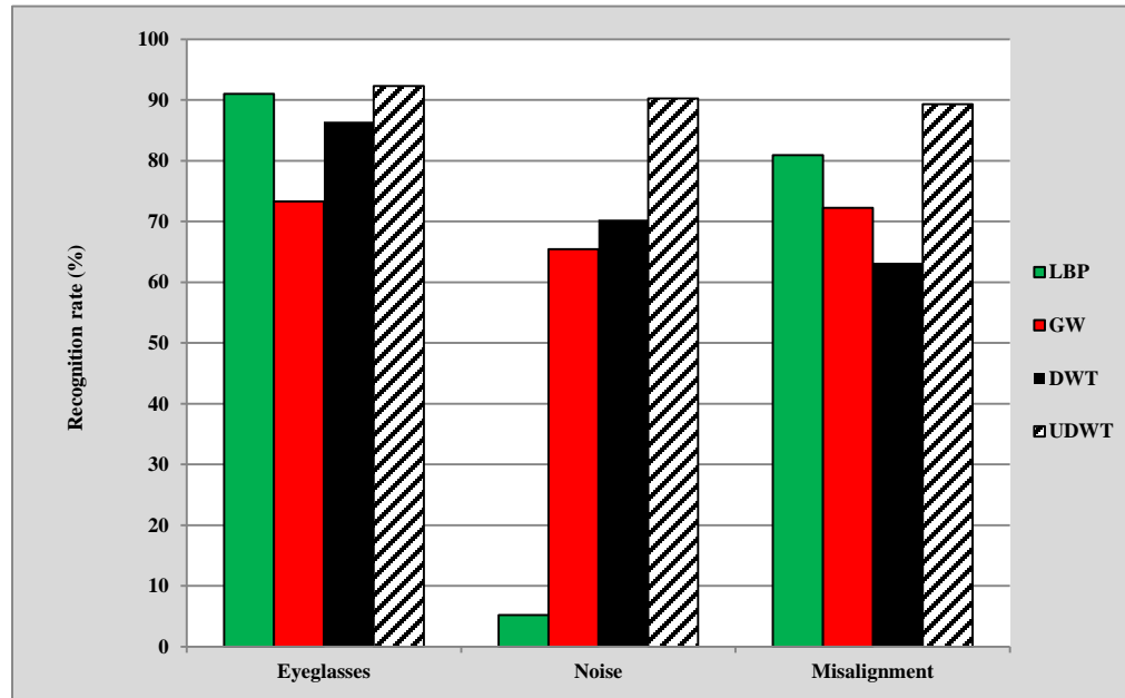
Figure 9 The performances of different local methods in the presence of eyeglasses, noise and misalignment
