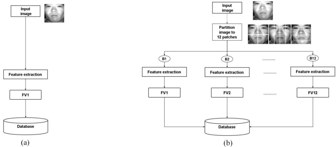
Figure 1 (a) The block diagram of global feature extraction (Training stage) (b) The block diagram of local feature extraction (Training stage)
