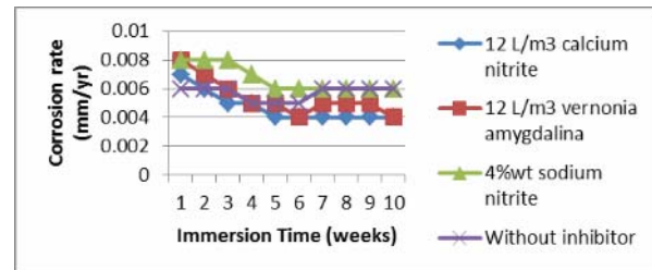
Figure-13. Corrosion rates (mm/yr) versus immersion time for carbon steel in concrete immersed in 3.5% NaCl solution.
