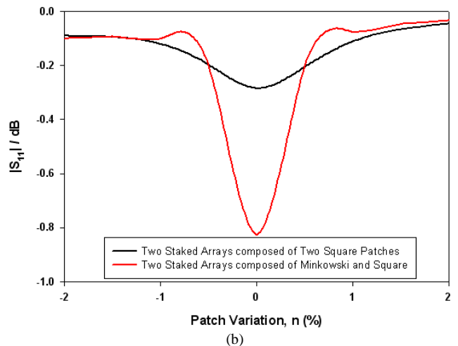
Figure 4 Simulation result for both purpose configurations. (a) Phase of the reflection coefficient. (b) Magnitude of the reflection coefficient
