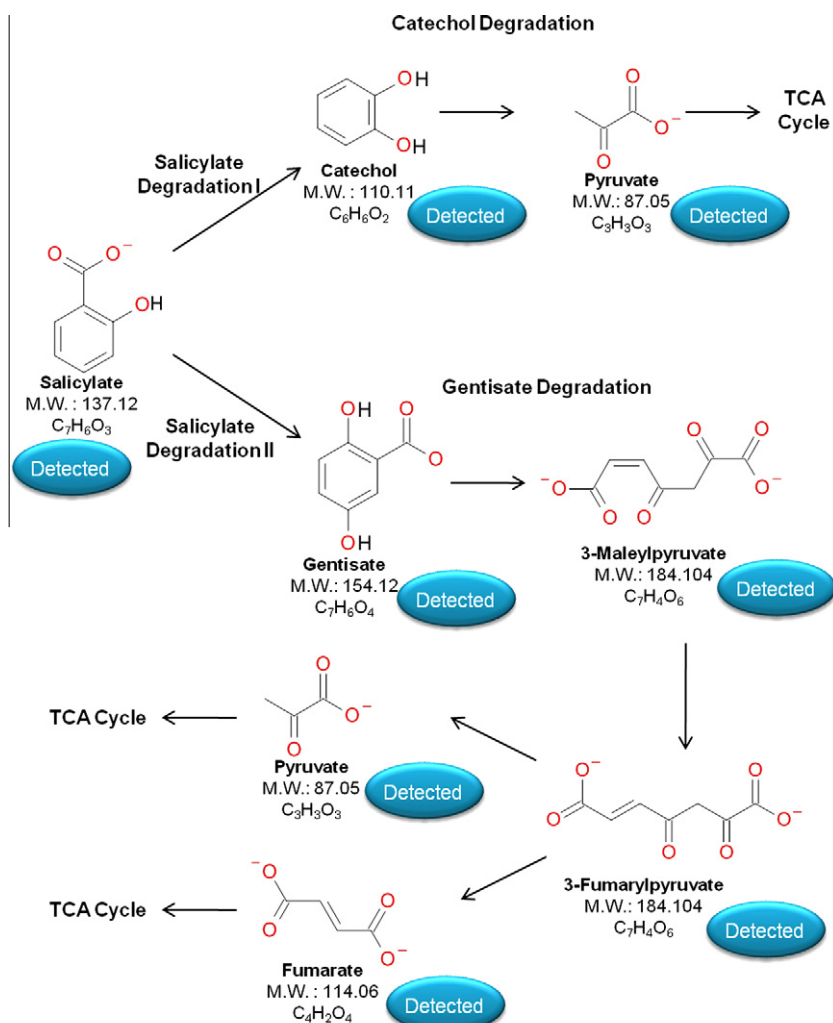
Fig. 6. Proposed salicylate degradation pathways by NAR-2 bacterial consortium.
