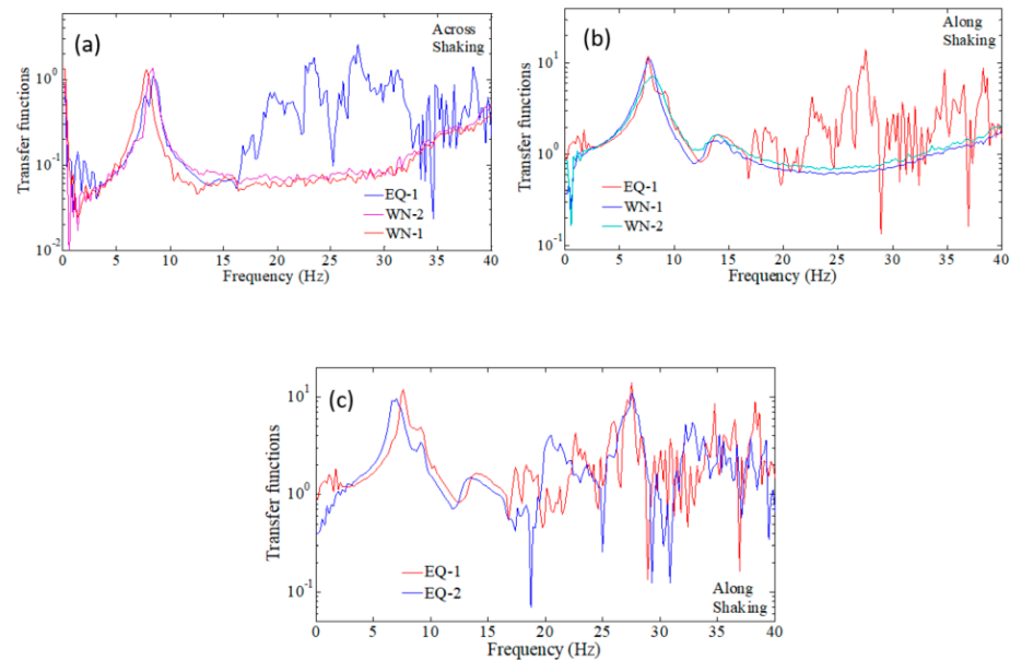
Figure 30. Transfer function estimates for the (a) across shaking direction during the loading states EQ-1, WN-1, WN-2; (b) along shaking direction during EQ-1, WN-1, WN-2; (c) along shaking direction during EQ-1, EQ-2.
