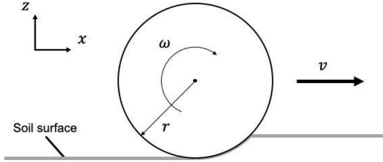
Fig. 2. Longitudinal wheel slip on loose soil.
