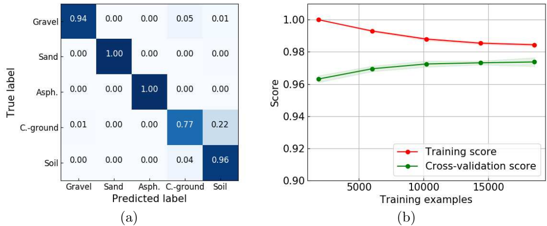
Fig. 11. Summary of ability and validity of terrain classifier. (a) Confusion matrix of terrain classifier with normalization. (b) Learning curve of terrain classifier. Green and red lines indicate the cross-validation score and training score, respectively. Color bands around each line indicate standard deviation of their scores.
